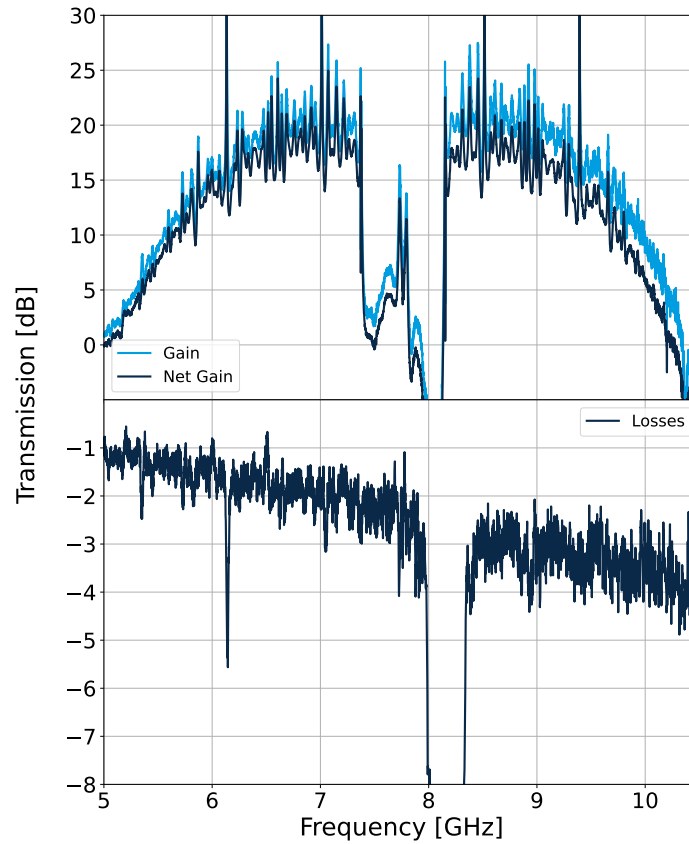
Figure 2: Top panel shows the gain (ON-OFF) and net gain (ON-lossless reference) of the TWPA. The pump parameters are (at the input of the TWPA): 7.764 GHz and -66.3 dBm. Bottom panel shows the electrical losses within the TWPA. The gap is centered at 8.15 GHz and is 0.41 GHz wide, the signal cannot propagate in the gap.
