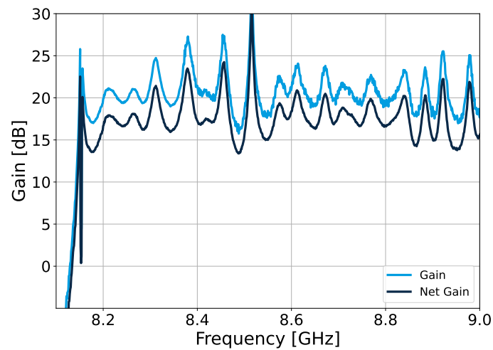
Figure 4: Zoom on the gain (ON-OFF) and net gain (ON-lossless reference) of the TWPA. The pump parameters are (at the input of the TWPA): 7.764 GHz and -66.3 dBm.
