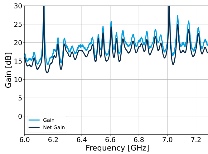
Figure 3: Zoom on the gain (ON-OFF) and net gain (ON-lossless reference) of the TWPA. The pump parameters are (at the input of the TWPA): 7.764 GHz and -66.3 dBm.
