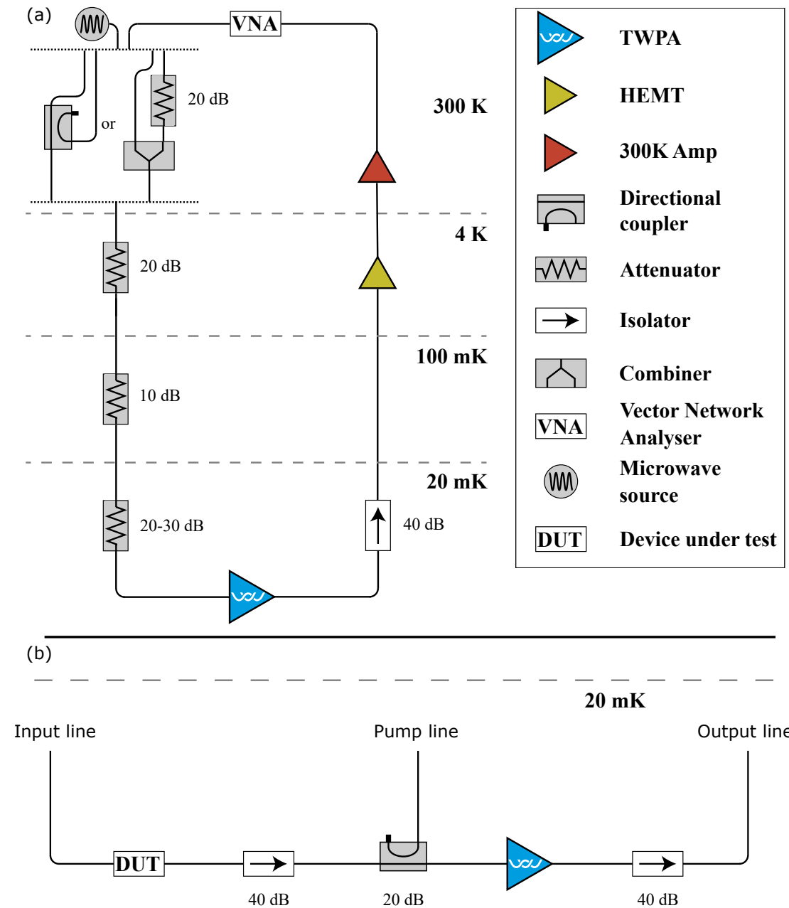
Figure 1: Typical setups for testing/using the TWPA. (a) Ideal setup for testing the TWPA. (b) TWPA in a readout line (at the mixing chamber stage). Note: always verify the directionnall coupler specifications to see which port is coupled to which port.
